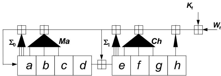
Figure 2 : Hash computation, state register update function
